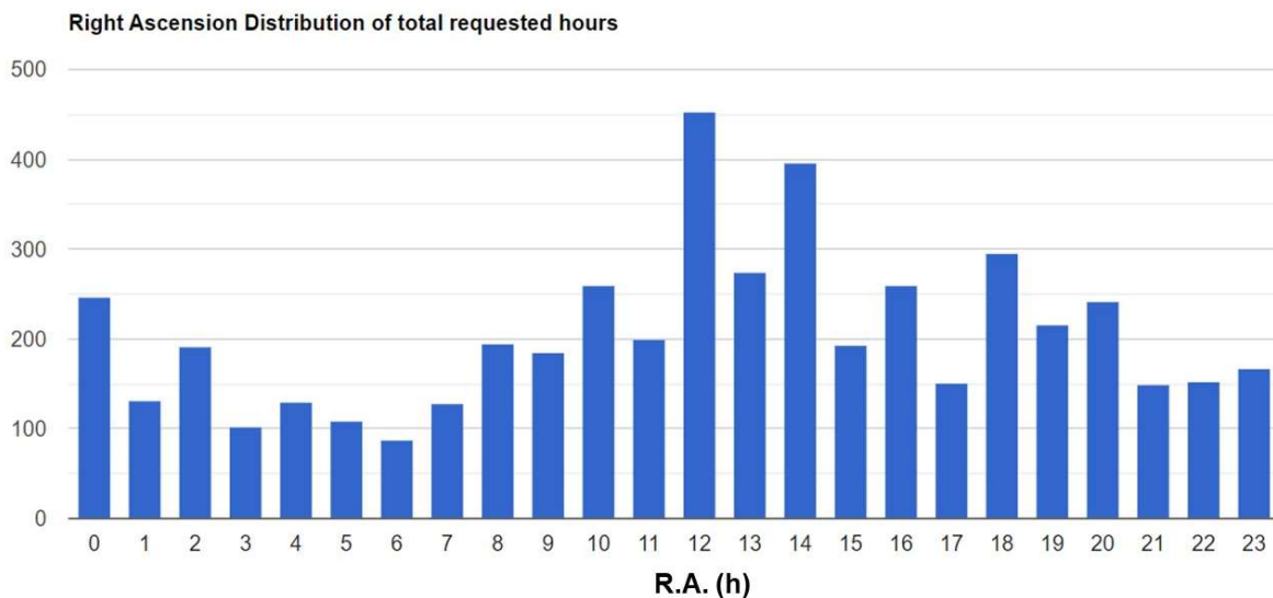
Figure 1: R.A. distribution for OBs that were requested to be executed in S22A+S22B. Note the high oversubscription in RA=12-14h and the relatively low demand for RA=19-23h.
